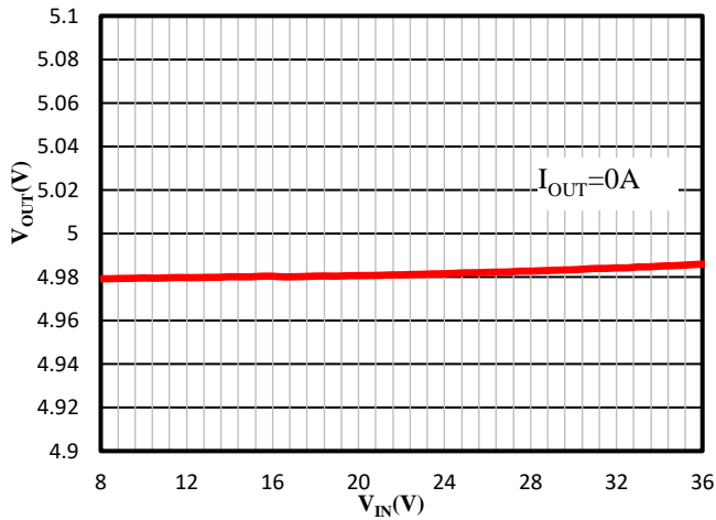
Figure 3. Line Regulation
