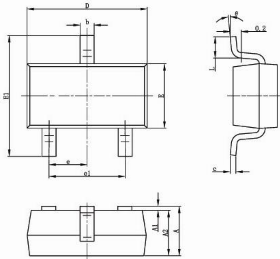
SOT-23-3L PACKAGE OUTLINE DIMENSIONS
